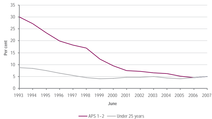
Figure 10: Ongoing staff: representation of APS 1–2s and employees aged under 25, 1993 to 2007
